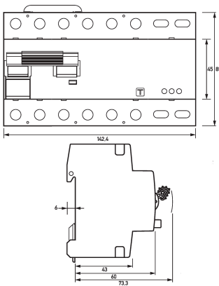
Dimensional drawing Group view
